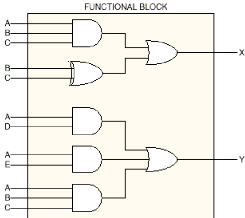
Figure 3-4. Schematic without Intermediate Signal
