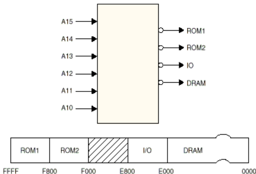
Figure 4-1. Block Diagram: Memory Address Decoder
