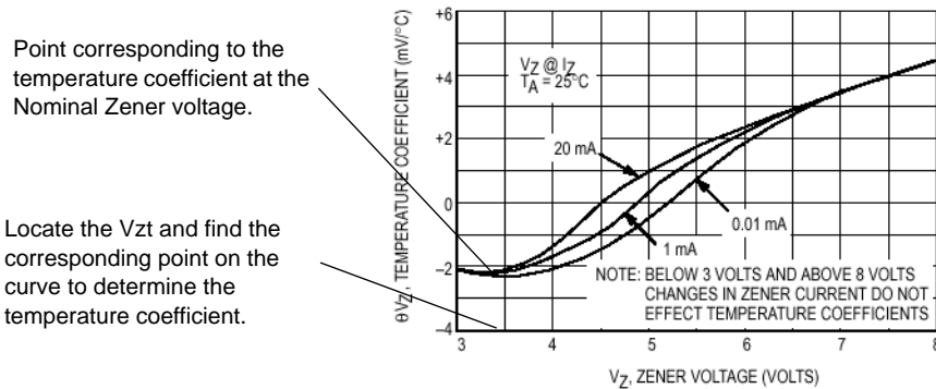
Figure 4. Effect of Zener Current
