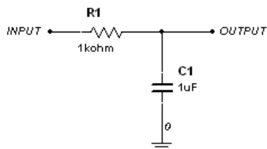
Figure P1a (Circuit)
